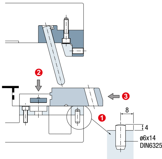
Mold Open
